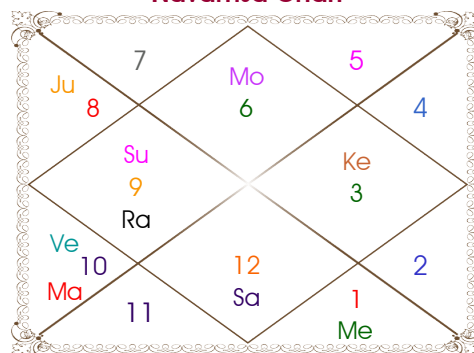
Navamsa Chart
